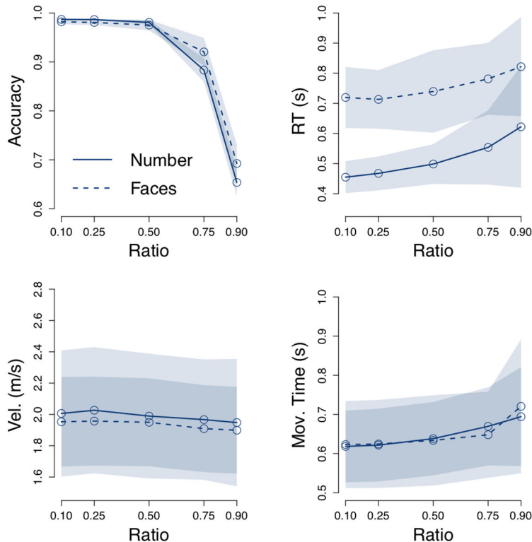
Figure 3. Performance and kinematics. Shading represents 2 s.e.m.
